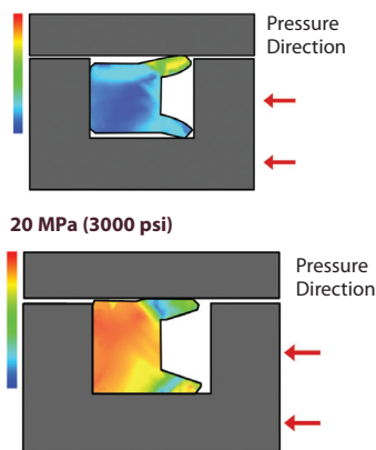
Figure 1. How the 22K performs installed and under pressure
