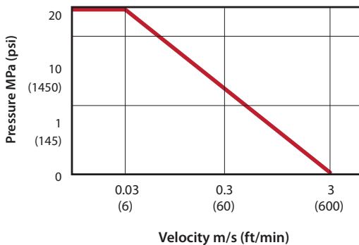
POLY-ACETAL PV (PRESSURE-VELOCITY) CHART
